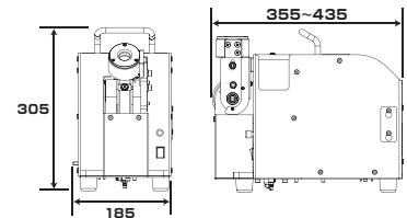
■ Dimensional drawing (unit: mm)
